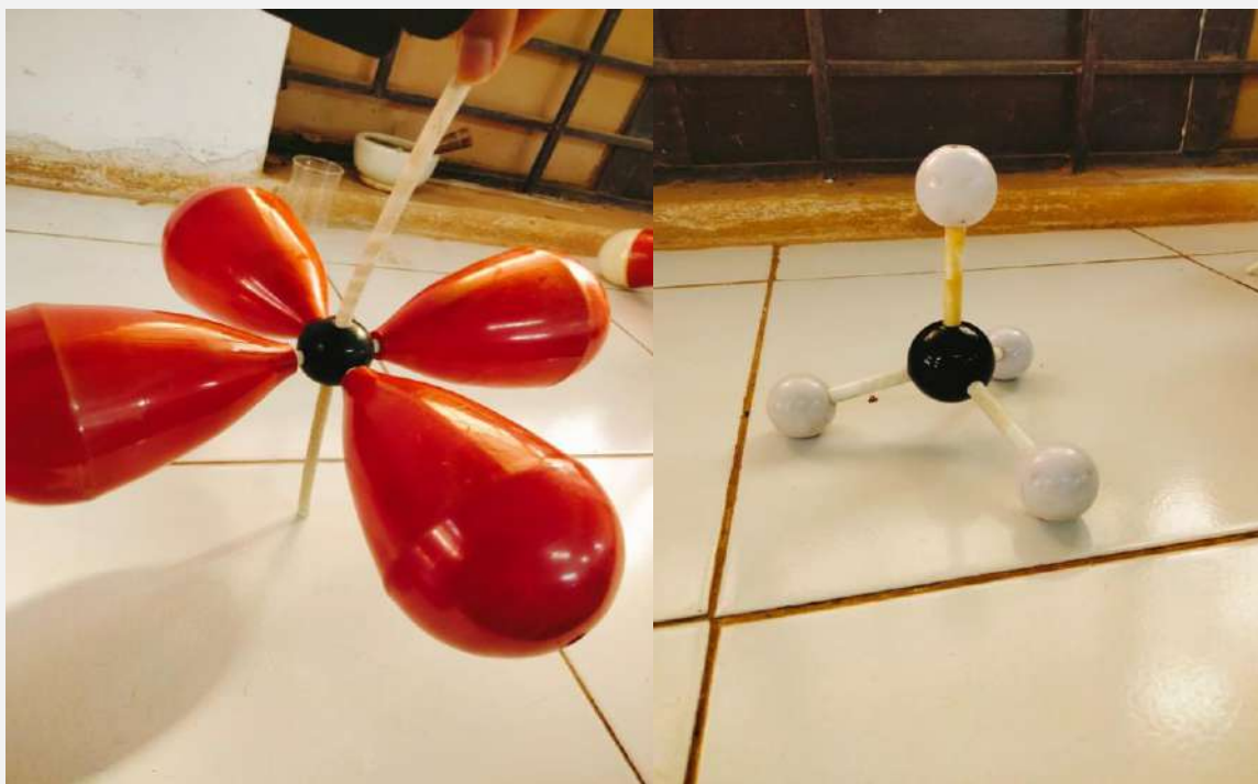
d_{x^2-y^2}
