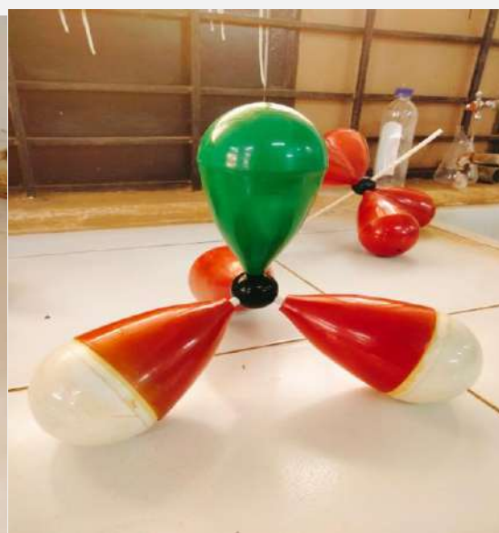
NH_3 Molecule
